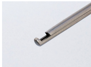
Small-Handle Punch, 250x3mm, 40° up-angled
