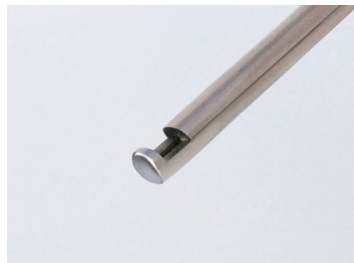
Ferris-Smith Punch, 180x4mm, 40° up-angled
