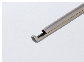
Sm-Hdl Punch, Lf-Handled Bayonet, 180x3mm, 40°
